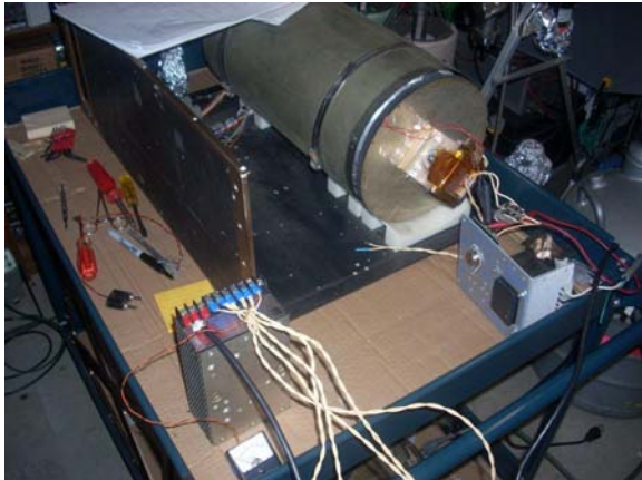
Getting ready to energize ovens
