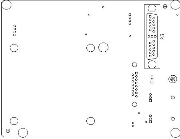
E193B-20007 REV C COMPONENT LOCATOR BOTTOMSIDE 05/21/97
